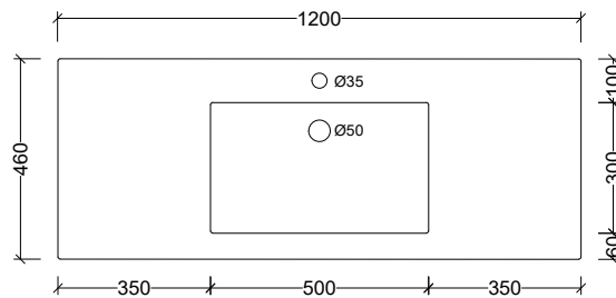
MMA120C Note: 1, 3, or 0 taphole available Available with overflow – see page 48.
