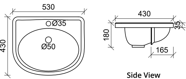
SFBBASC Note: 1, 3, or 0 taphole available Available with overflow – see page 48.
