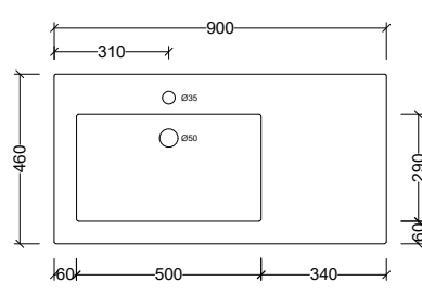
ESS900 Note: 1, 3, or 0 taphole available LH or RH offset. Available with overflow – see page 48.
