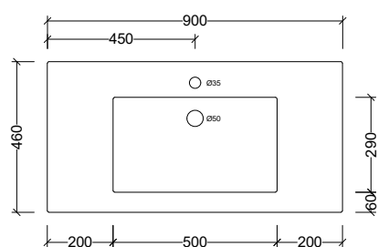
ESS900C Note: 1, 3, or 0 taphole available Available with overflow – see page 48.
