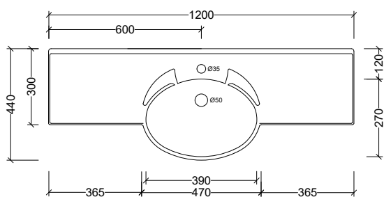
SFB120C Note: 1, 3, or 0 taphole available Available with overflow – see page 48.
