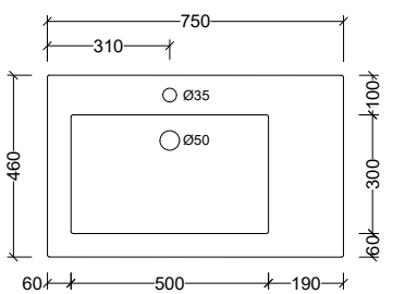
MGR750 Note: 1, 3, or 0 taphole available
