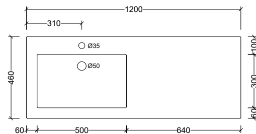
MMA120 Note: 1, 3, or 0 taphole available LH or RH offset Available with overflow – see page 48.
