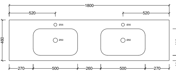
STA180D Note: 1, 3, or 0 taphole available
