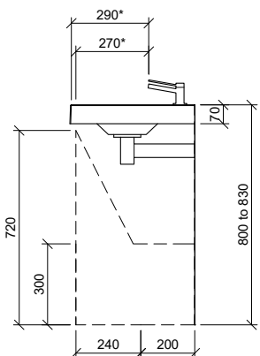
Side View - All Sizes
