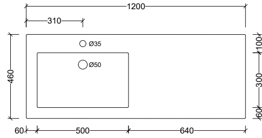
MGR120 Note: 1, 3, or 0 taphole available
