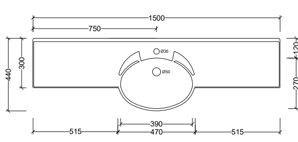
SFB150C Note: 1, 3, or 0 taphole available Available with overflow – see page 48.
