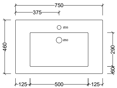
ESS750C Note: 1, 3, or 0 taphole available Available with overflow – see page 48.
