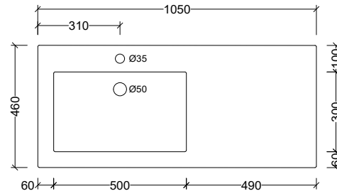
MMA105 Note: 1, 3, or 0 taphole available LH or RH offset Available with overflow – see page 48.
