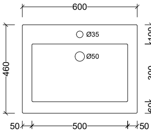
MGR600C Note: 1, 3, or 0 taphole available
