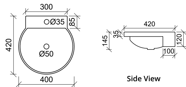
QFBBASC Note: 1, 3, or 0 taphole available Available with overflow – see page 48.
