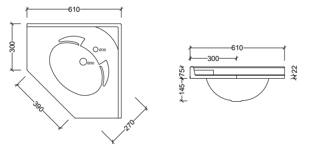
SCN610C Note: 1, 3, or 0 taphole available Available with overflow – see page 48.
