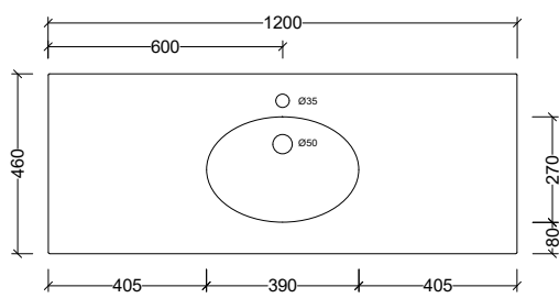
ELI120C Note: 1, 3, or 0 taphole available Available with overflow – see page 48.
