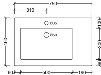
MMA750 Note: 1, 3, or 0 taphole available LH or RH offset Available with overflow – see page 48.
