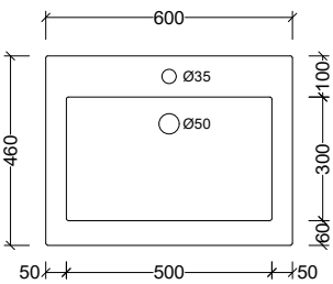
MMA600C Note: 1, 3, or 0 taphole available Available with overflow – see page 48.
