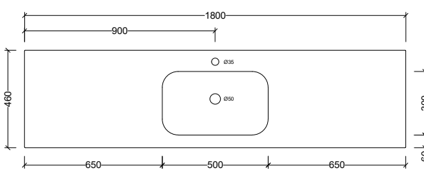
STA180C Note: 1, 3, or 0 taphole available
