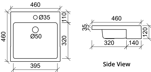
CFB460C Note: 1, 3, or 0 taphole available Available with overflow – see page 48.
