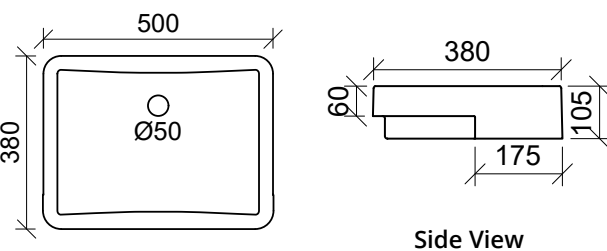
FFB175C0 Note: 0 taphole available
