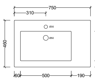
ESS750 Note: 1, 3, or 0 taphole available LH or RH offset. Available with overflow – see page 48.
