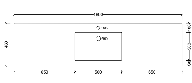
MGR180C Note: 1, 3, or 0 taphole available
