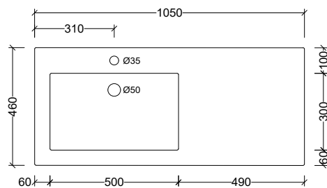
MGR105 Note: 1, 3, or 0 taphole available
