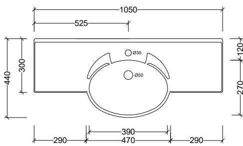
SFB105C Note: 1, 3, or 0 taphole available Available with overflow – see page 48.
