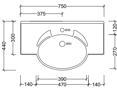
SFB750C Note: 1, 3, or 0 taphole available Available with overflow – see page 48.
