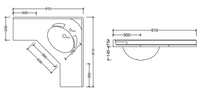
SCN910C Note: 1, 3, or 0 taphole available Available with overflow – see page 48.
