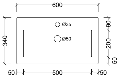
MGE600C Note: 1, 3, or 0 taphole available Available with overflow – see page 48.
