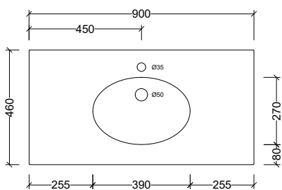
ELI900C Note: 1, 3, or 0 taphole available Available with overflow – see page 48.
