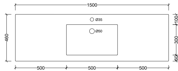
MMA150C Note: 1, 3, or 0 taphole available Available with overflow – see page 48.
