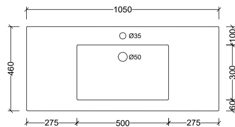
MMA105C Note: 1, 3, or 0 taphole available Available with overflow – see page 48.
