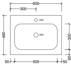
STA600C Note: 1, 3, or 0 taphole available
