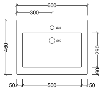
ESS600C Note: 1, 3, or 0 taphole available Available with overflow – see page 48.
