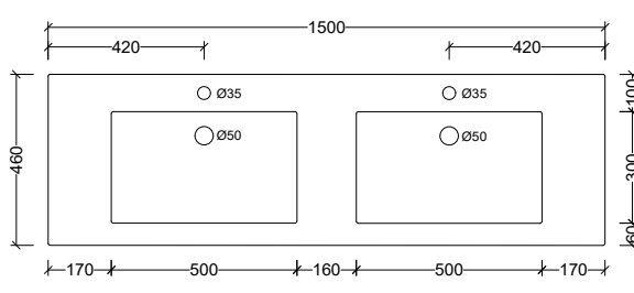
MGR150D Note: 1, 3, or 0 taphole available
