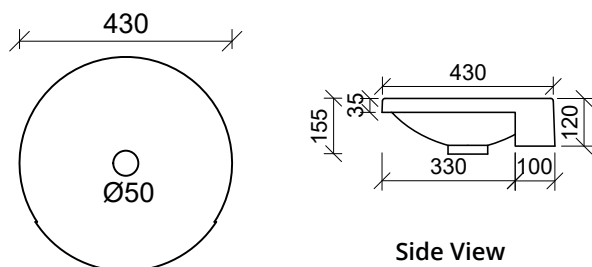
CFB120C0 Note: 0 taphole available
