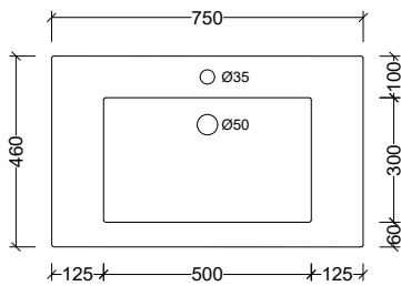
MMA750C Note: 1, 3, or 0 taphole available Available with overflow – see page 48.
