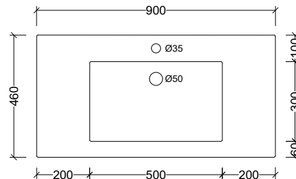
MMA900C Note: 1, 3, or 0 taphole available Available with overflow – see page 48.
