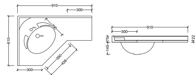
SCN910 Note: 1, 3, or 0 taphole available LH or RH offset Available with overflow – see page 48.
