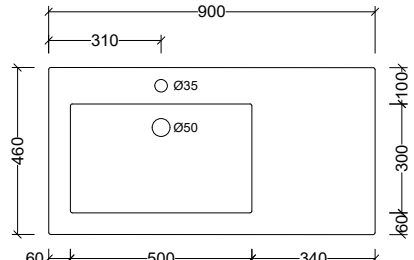
MMA900 Note: 1, 3, or 0 taphole available LH or RH offset Available with overflow – see page 48.
