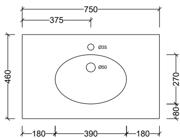
ELI750C Note: 1, 3, or 0 taphole available Available with overflow – see page 48.
