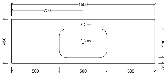
STA150C Note: 1, 3, or 0 taphole available
