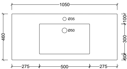
MGR105C Note: 1, 3, or 0 taphole available
