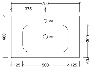
STA750C Note: 1, 3, or 0 taphole available
