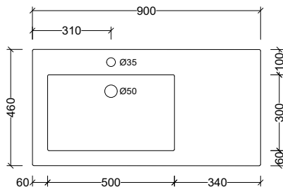
MGR900 Note: 1, 3, or 0 taphole available
