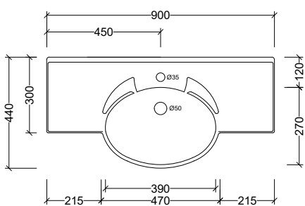
SFB900C Note: 1, 3, or 0 taphole available Available with overflow – see page 48.
