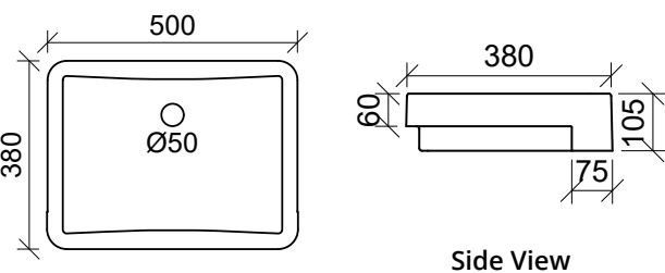
FFB075C0 Note: 0 taphole available
