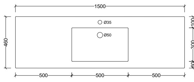
MGR150C Note: 1, 3, or 0 taphole available
