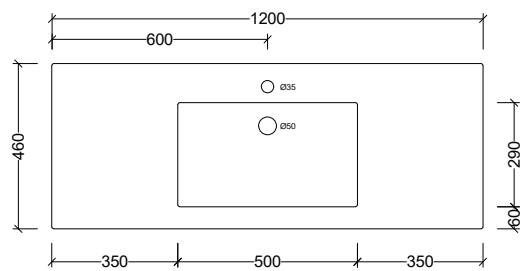
ESS120C Note: 1, 3, or 0 taphole available Available with overflow – see page 48.
