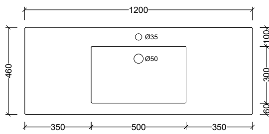
MGR120C Note: 1, 3, or 0 taphole available
