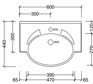
SFB600C Note: 1, 3, or 0 taphole available Available with overflow – see page 48.
