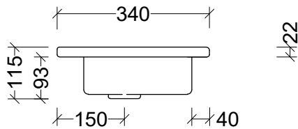
Side View - All Sizes
