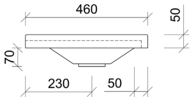
Side View - All Sizes
