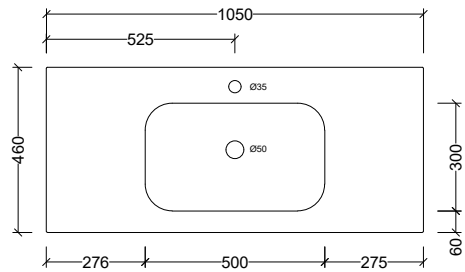
STA105C Note: 1, 3, or 0 taphole available
